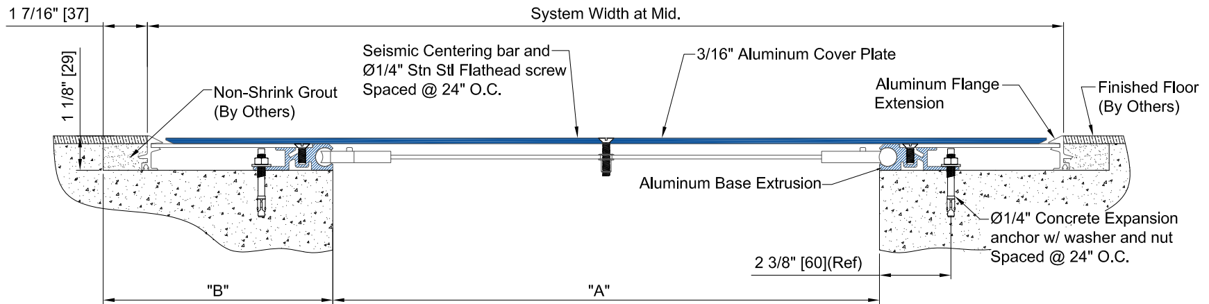
FNB-1800 DETAIL Floor to Floor Condition
