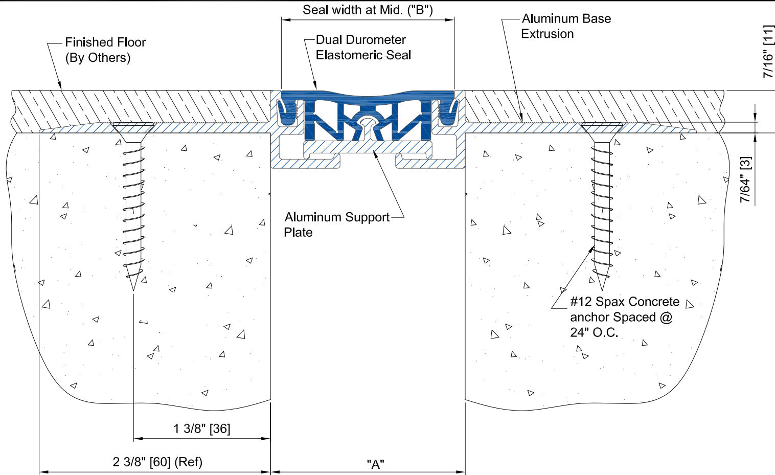
CWFC-200 thru 300 DETAIL FLOOR TO FLOOR CONDITION
