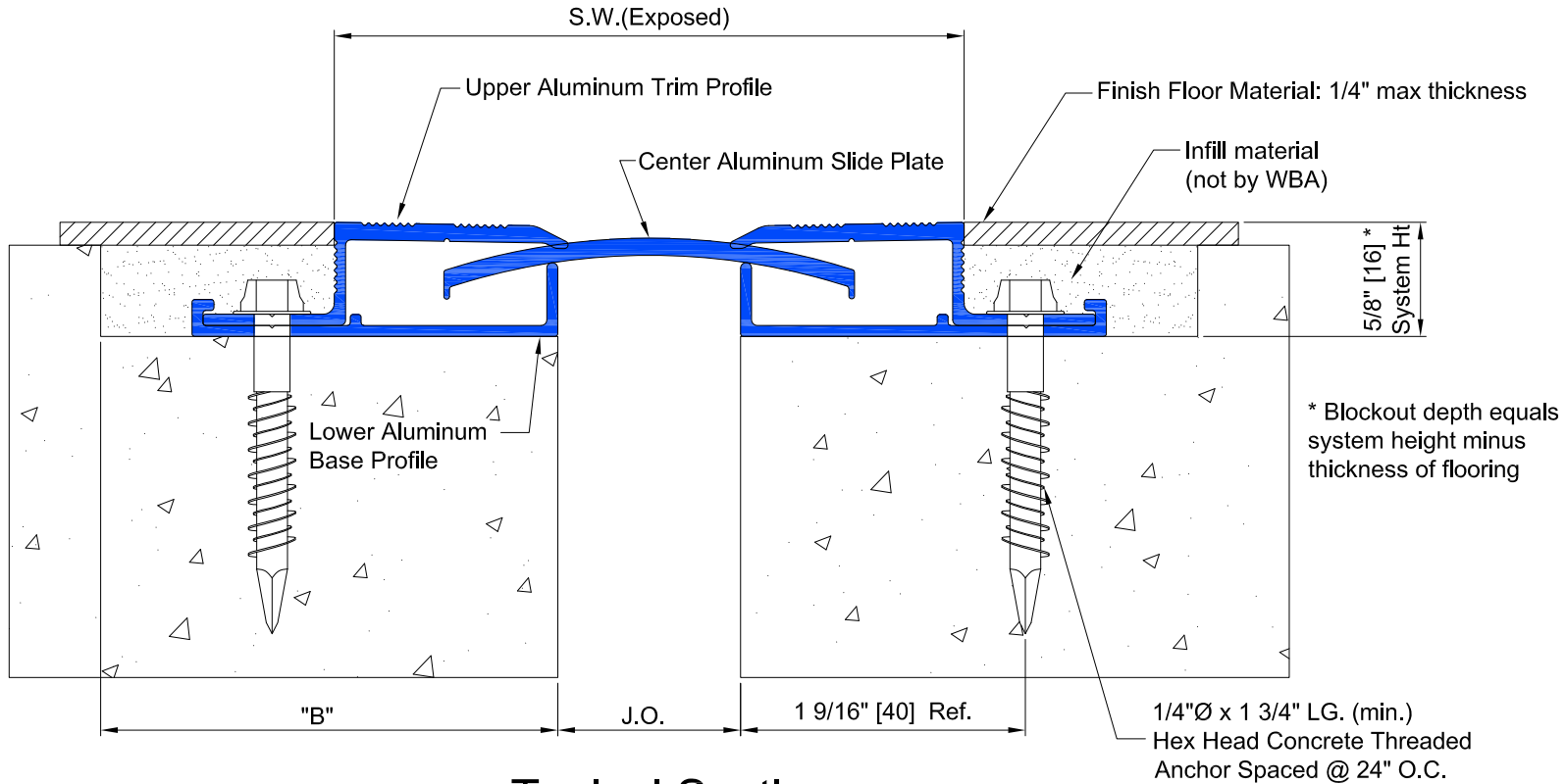
Typical Section Floor To Floor
