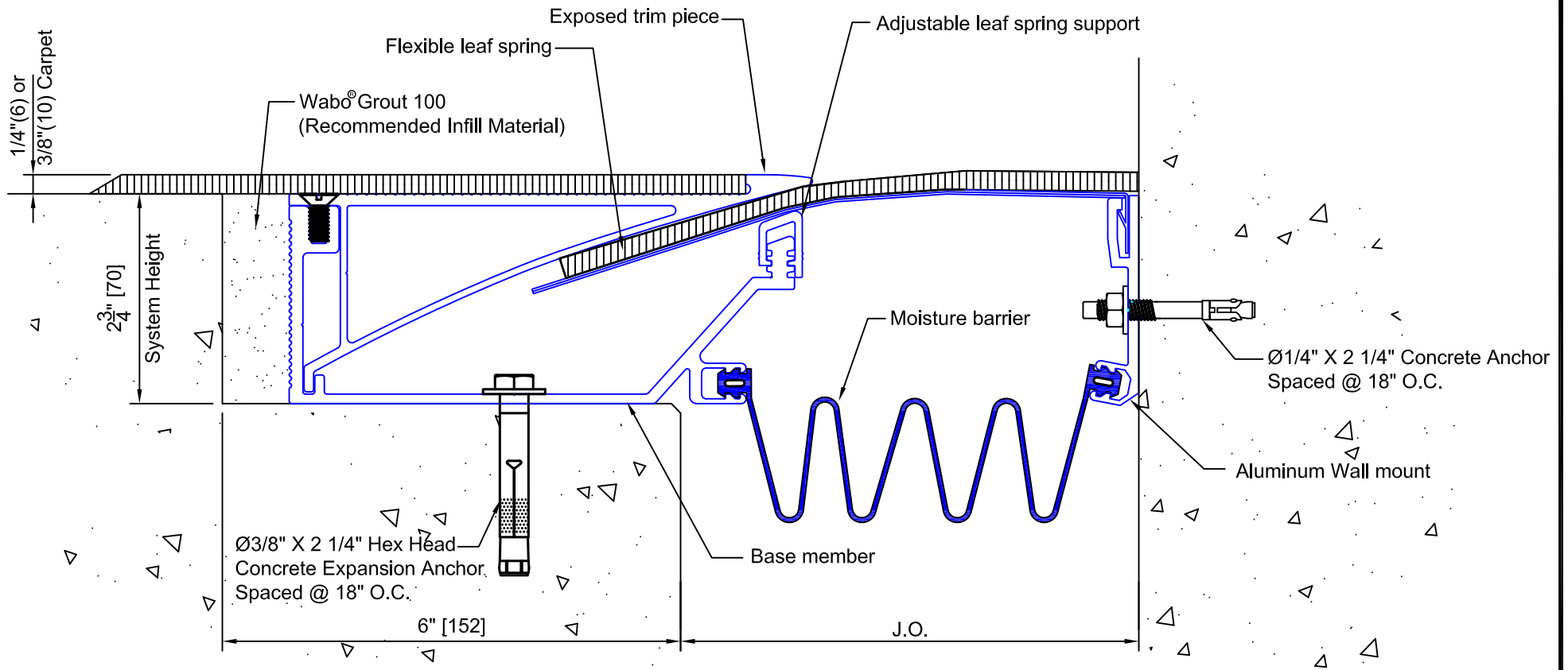
Typical Detail Floor to Wall - Carpet Condition
