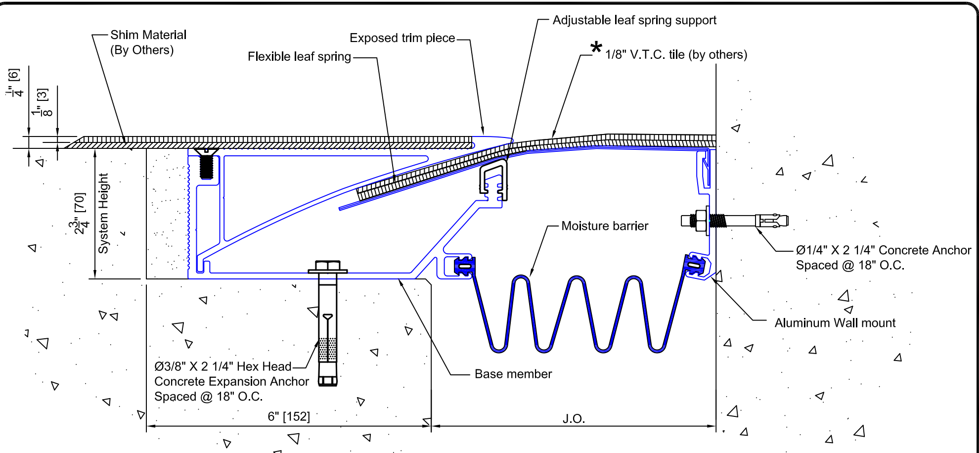
Typical Detail Floor to Wall - Tile Condition
