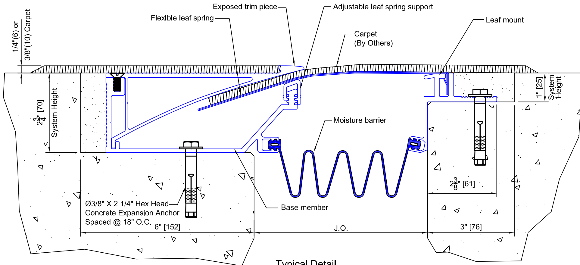
Typical Detail Floor to Floor - Carpet Condition
